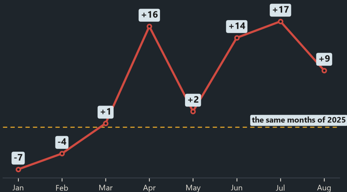
PM10 monthly mean residual, \mu\text{g}/\text{m}^3 against 2025
