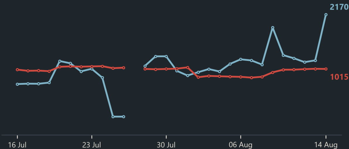
CO, daily level, not a residual (µg/m³)
