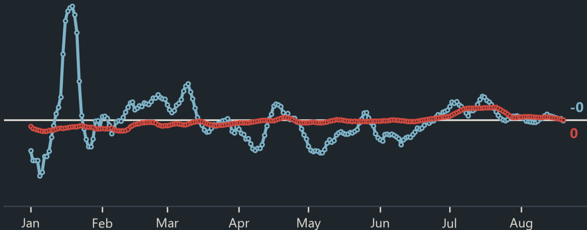
PM10 residual, 2026
