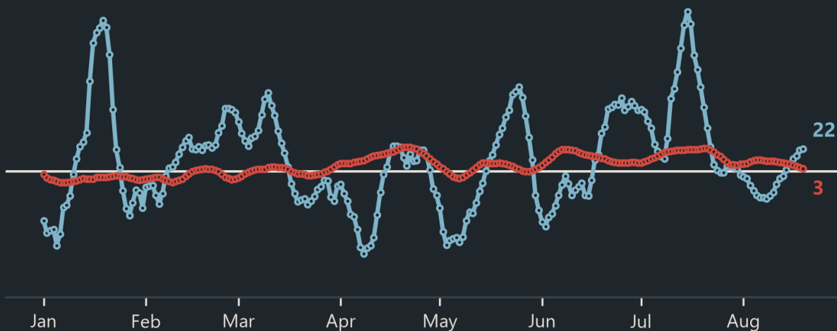
PM10 residual, 2026
