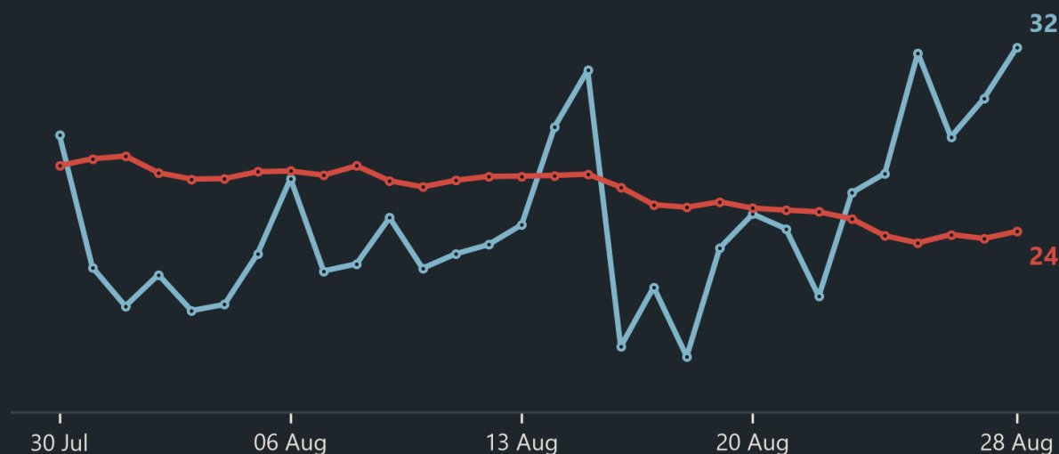
NO 2 , daily level, not a residual (µg/m 3 )
