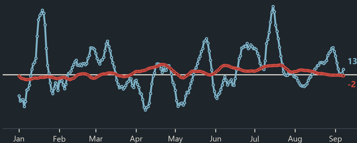
PM10 residual, 2026
